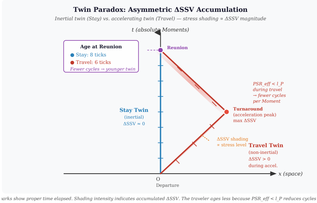
Figure 3: Twin paradox: asymmetric \Delta\text{SSV} accumulation along inertial vs. non-inertial world-lines. The stay twin (blue vertical line) remains inertial throughout; \Delta\text{SSV} \approx 0 so \text{PSR}_{\text{eff}} = l_P and clock ticks (horizontal marks) are evenly spaced in absolute time. The travel twin (red diagonal) accelerates outward, turns around, and returns; the shading intensity along the worldline is proportional to the accumulated \Delta\text{SSV} . Because \text{PSR}_{\text{eff}} < l_P during travel, each displacement step is shorter and more absolute Moments are required per oscillation cycle. The travel twin, therefore, records fewer proper-time ticks (6 vs. 8 shown) and is younger at reunion (purple circle). The asymmetry is physical, not a reciprocal illusion: only the travel twin accumulates \Delta\text{SSV} from acceleration, distinguishing CPP’s mechanistic resolution from purely geometric spacetime arguments.
