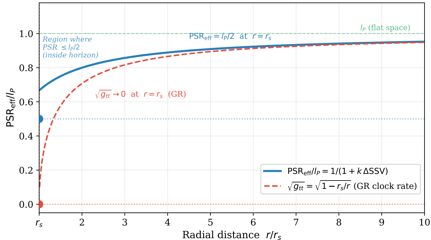
Figure 3. PSR contraction approaching the Schwarzschild horizon. The CPP Planck cutoff at \text{PSR}_{\text{eff}} = l_P/2 prevents the GR singularity.
