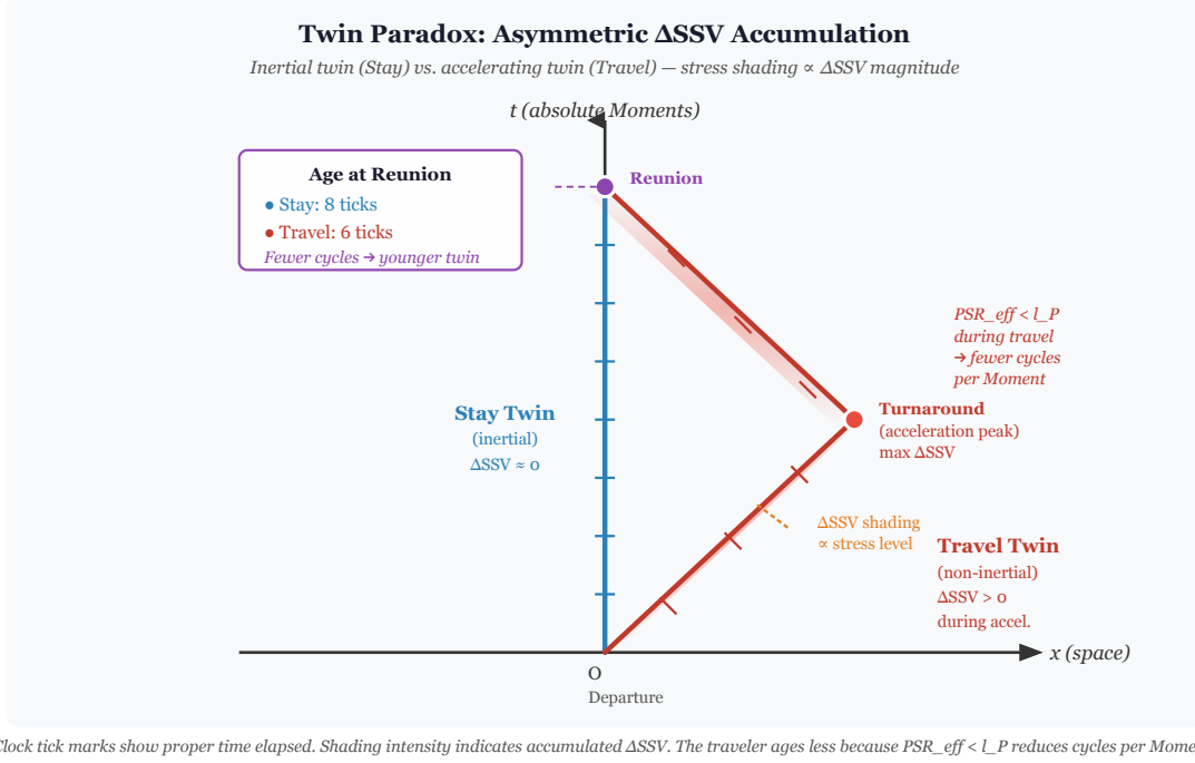
Figure 3: Twin paradox: asymmetric \Delta SSV accumulation along inertial vs. non-inertial world-lines. The stay twin (blue vertical line) remains inertial throughout; \Delta SSV \approx 0 so PSR_{eff} = l_P and clock ticks (horizontal marks) are evenly spaced in absolute time. The travel twin (red diagonal) accelerates outward, turns around, and returns; the shading intensity along the worldline is proportional to the accumulated \Delta SSV. Because PSR_{eff} < l_P during travel, each displacement step is shorter and more absolute Moments are required per oscillation cycle. The travel twin, therefore, records fewer proper-time ticks (6 vs. 8 shown) and is younger at reunion (purple circle). The asymmetry is physical, not a reciprocal illusion: only the travel twin accumulates \Delta SSV from acceleration, distinguishing CPP’s mechanistic resolution from purely geometric spacetime arguments.
