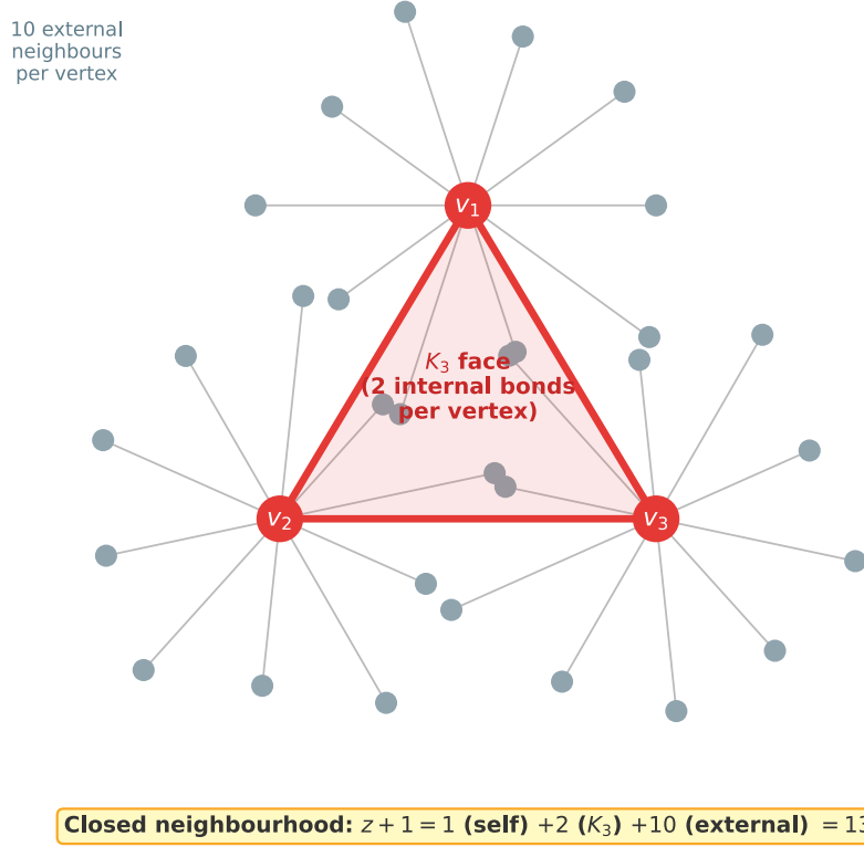
Figure 3: A K_3 face (red triangle, vertices v_1, v_2, v_3 ) embedded in the 600-cell lattice. Each vertex has 2 internal bonds (red, to K_3 partners) and 10 external bonds (grey, to the rest of the lattice). The closed neighbourhood has z + 1 = 1 (self) + 2 ( K_3 ) + 10 (external) = 13 sites. The isotropic EW perturbation \varepsilon is the abelian energy from the 2 internal bonds, normalised by the 13-site closed neighbourhood.
