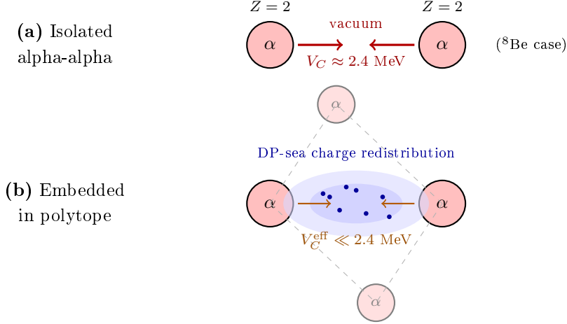
Figure 4: Schematic representation of alpha-alpha Coulomb behavior in two regimes. (a) Isolated alpha-alpha contact (top): the ^8\text{Be} case, where two alphas interact without neighbors; full vacuum Coulomb repulsion V_C \approx 2.4 \text{ MeV} operates, extracted from the observed 92 keV unboundness (Finding 4.1). (b) Alpha-alpha contact embedded in a larger polytope (bottom): with additional alpha neighbors present (gray, dashed edges), the DP-sea between the two central alphas reorganizes to partially screen the local charge product; effective Coulomb V_C^{\text{eff}} becomes substantially reduced from 2.4 MeV. This figure is a schematic representation of the screening mechanism proposed in the text; it does not depict a derived DP-sea charge distribution. A first-principles CPP derivation of the DP-sea screening profile is deferred to future work (OPEN-SS-22-adjacent, targeted for SS-8). The empirical evidence for reduced effective Coulomb in the embedded regime is the Table 1 agreement of the Coulomb-free formula within \pm 1.5\% , contrasted with the full-Coulomb ^8\text{Be} analysis of §4.
