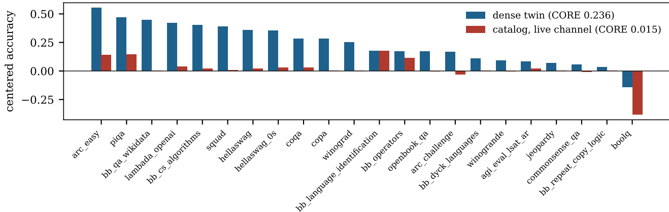
nanochat d20, 4980 steps, same data/silicon: CORE per task
