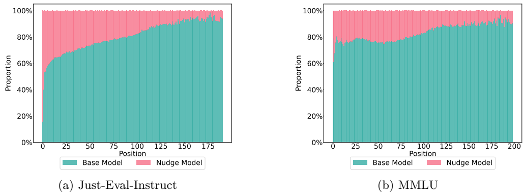
Figure 17: Nudging Ratio Histogram.
