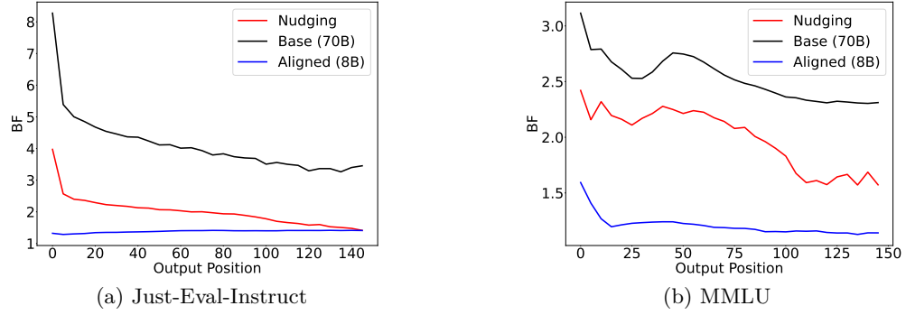
Figure 16: Output Perplexity Dynamics in Nudging Experiments.
