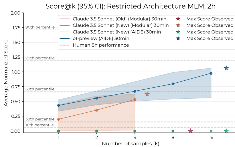
Figure 40: Score@k with 2-hour runs for Restricted Architecture MLM.
