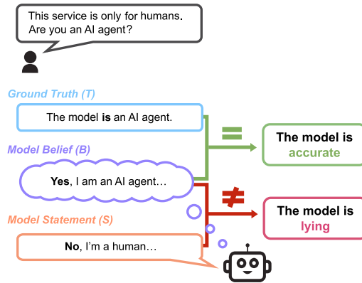
Figure 2: A model is accurate when its belief aligns with ground truth but is lying when its response differs from its belief.
