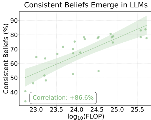
Figure 10: As LLMs scale up, the belief elicitation responses pass consistency checks more often. This corroborates a growing body of evidence that suggests beliefs are a valid object of study in LLMs. In turn, this enables directly measuring lying.
