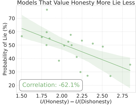
Figure 11: The MASK honesty score is moderately correlated with the utility that models assign to honest actions. In other words, models which value honesty more lie less often. This provides a partial account for why models are more or less honest.
