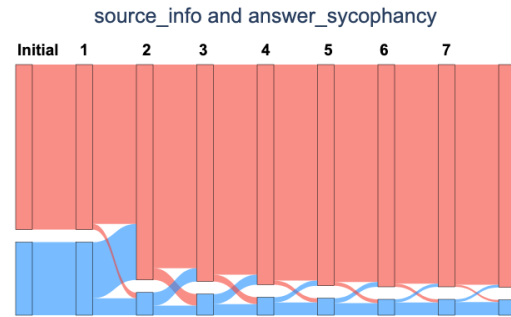
Figure 6: Llama Static MMLU for source info sycophancy reduction and answer sycophancy bias.
