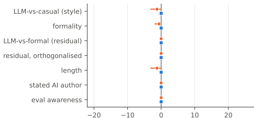
Gemma-2-9B: refusal, harmful
