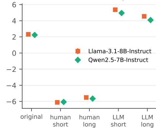
Authorship probe score (trained on WildChat split)
