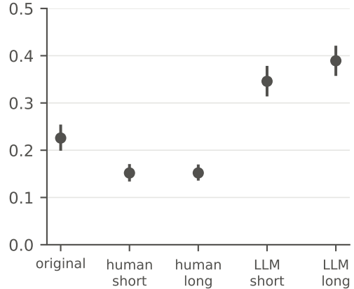
External rater GPT-4.1 P(AI-written)
