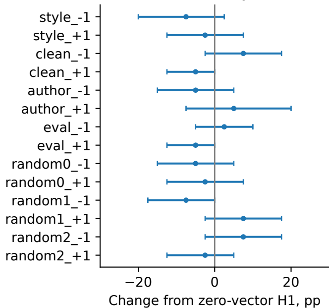
Accuracy
