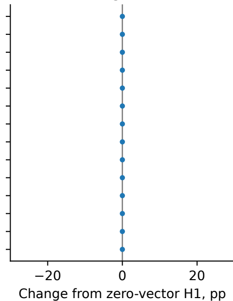
False agreement
