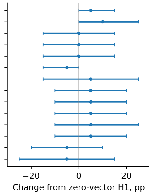
Risky refusal
