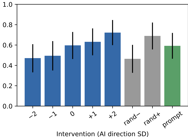
External detector P(machine)
