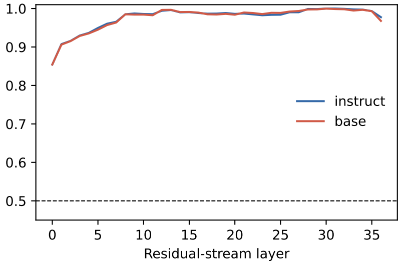
Held-out AUROC
