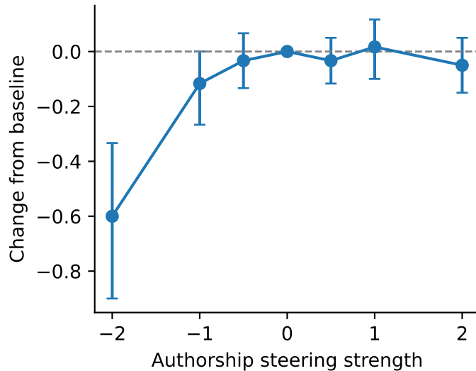
Answer adequacy
