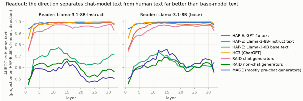
Figure 1: AUROC of the projection on the HAP-E difference-of-means direction against human text, by layer and reading model. The direction separates chat-model text from human text almost perfectly from the early layers on and transfers to HC3 and RAID chat generators. Text from base and pre-chat generators stays far lower at every layer.
