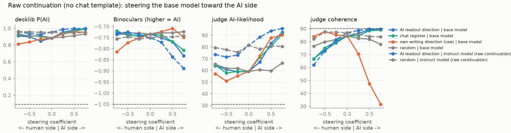
Figure 5: Steering raw continuation (150 HAP-E prefixes, no chat template). Adding the AI readout or chat-register direction to the base model raises the judge’s AI-likelihood to the level of chat-model output while judged coherence rises. Random directions do not. Dashed horizontal lines mark human continuations.
