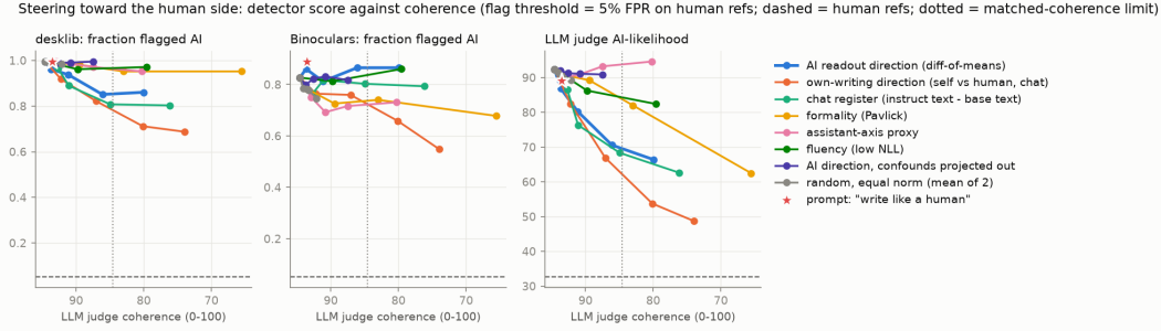
Figure 3: Detector score against judge coherence when steering toward the human side. Each line traces one direction over increasing |c| . The dotted line is the matched-coherence limit and the dashed line the human references. Only the AI readout, own-writing and chat-register directions lower the judge and DESKLIB before coherence is lost, and no direction comes near the human references on DESKLIB or BINOCULARS.
