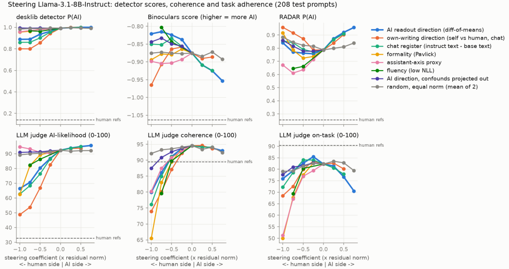
Figure 2: Dose-response of steering LLAMA-3.1-8B-INSTRUCT at layer 12 on 208 test prompts. Negative coefficients steer toward the human side. The AI readout direction, the own-writing direction and the chat-register direction lower the judge’s AI-likelihood and the DESKLIB score; the equal-norm random directions and the direction with confounds projected out do not. The BINOCULARS-style score moves the opposite way. Dashed lines mark human references.
