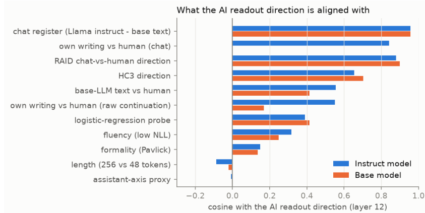
Figure 4: Cosine of each candidate direction with the AI readout direction at layer 12, in both models. Chat register is almost parallel to it; formality, length and the assistant-axis proxy are close to orthogonal.
