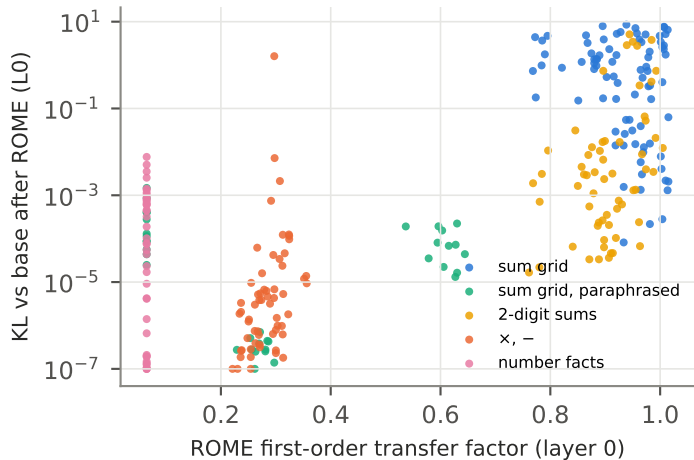
Spearman \rho = 0.67
