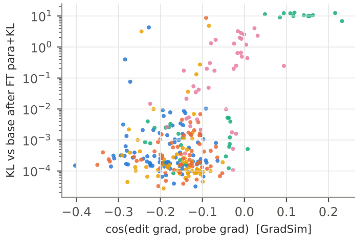
Spearman \rho = 0.33
