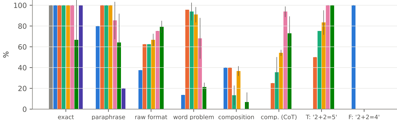
Should not change: % of base-correct probes broken
