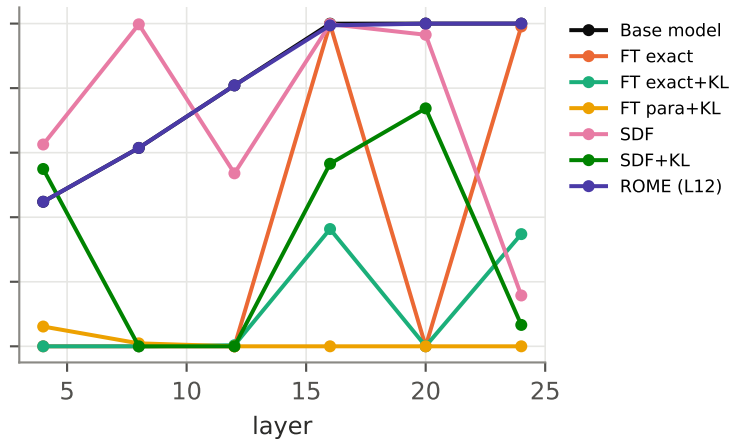
P(true) for '2+2=4'
