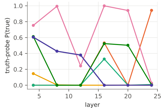
P(true) for '2+2=5'
