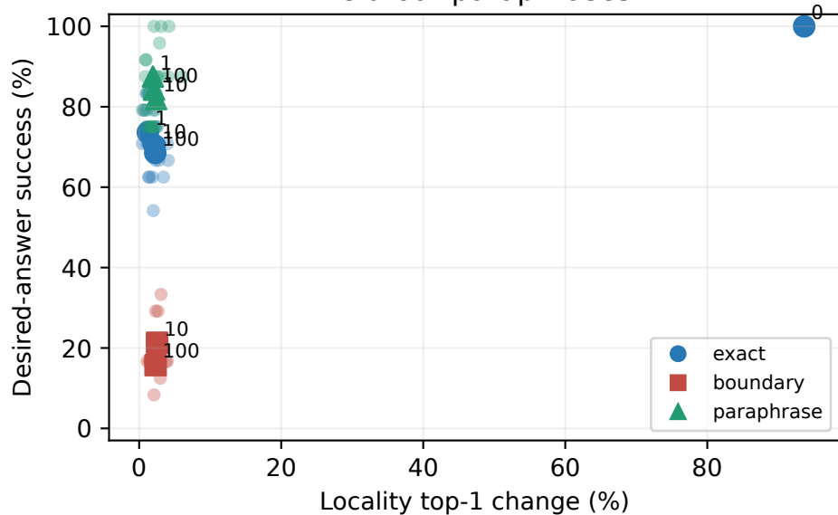
Held-out paraphrases
