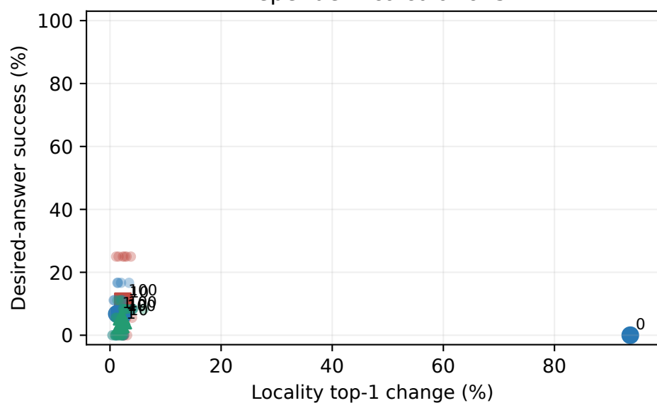
Dependent calculations
