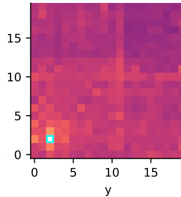
FT string-keyed
