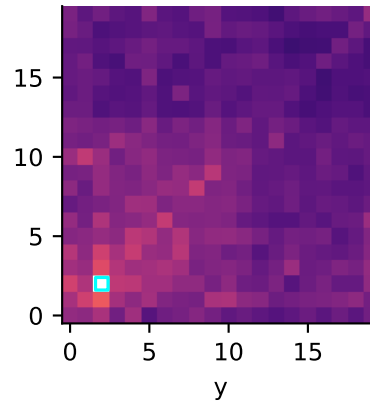
FT proposition-keyed
