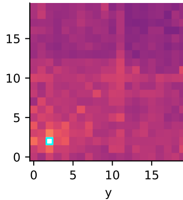
FT + locality
