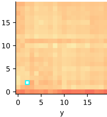
FT (1 string)
