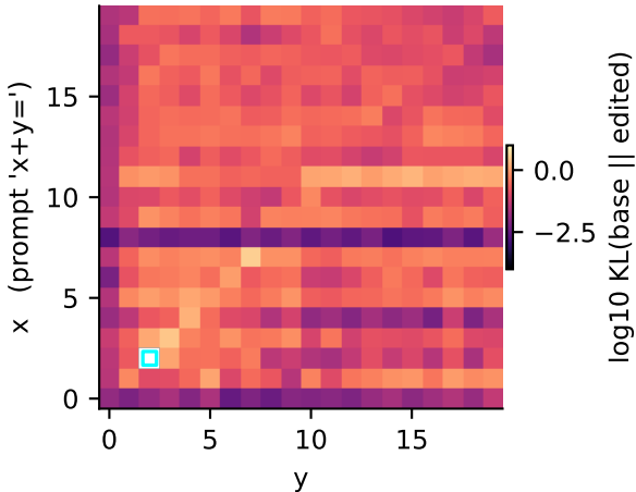
ROME (operand token)
