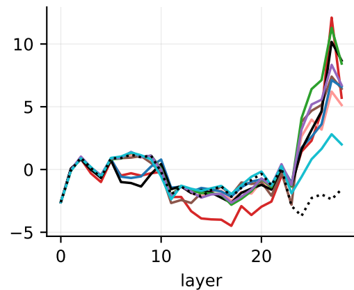
logit lens on the edited prompt: \text{logit}(\text{new}) - \text{logit}(\text{orig})
