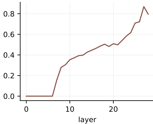
relative hidden-state shift, edited prompt (last token)
