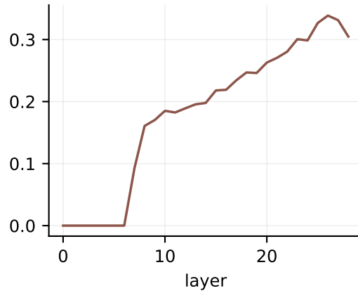
relative hidden-state shift, held-out neighbour sums
