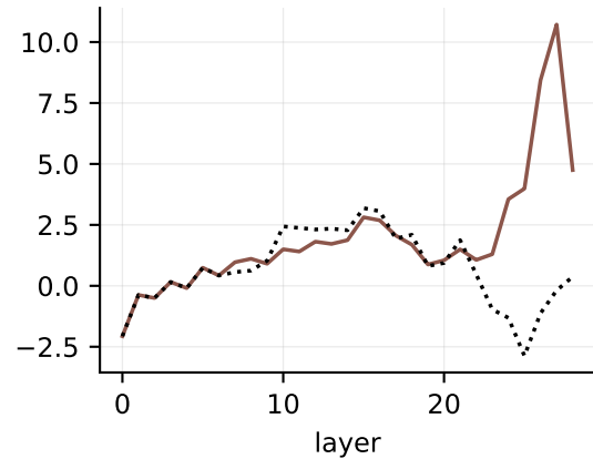
logit lens on the edited prompt: \text{logit}(\text{new}) - \text{logit}(\text{orig})
