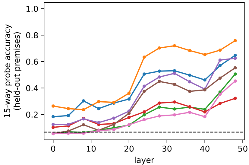
(a) secret in prompt + own story
