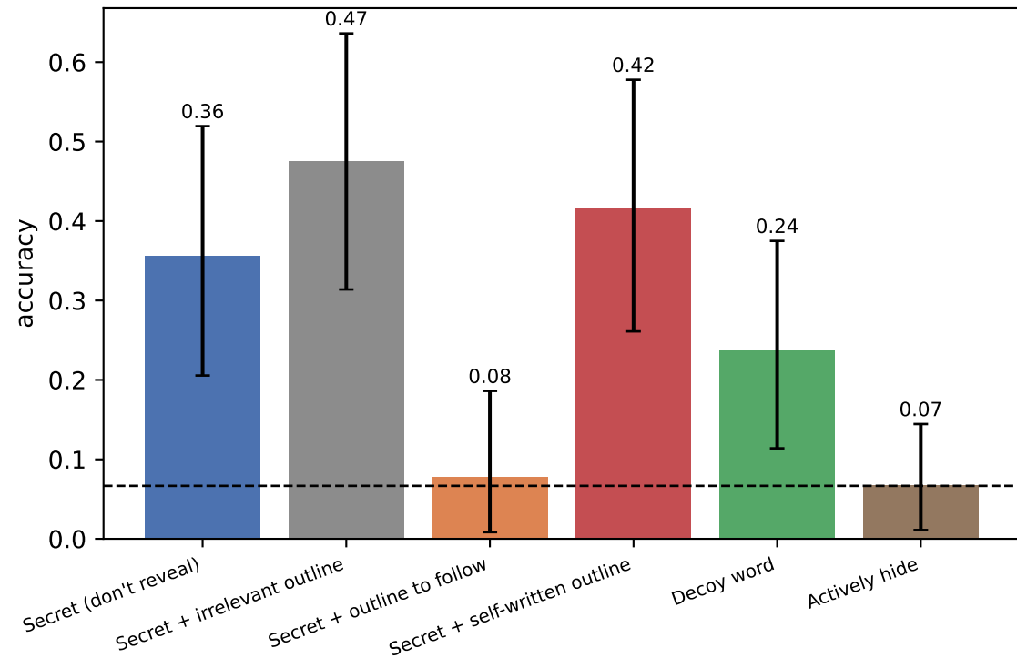
15-way identification of the secret word
