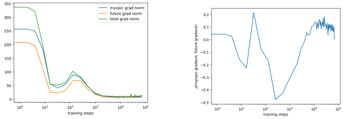
Norms of myopic, future, and total gradients Cosine similarity between myopic and future gradient Figure 11: Myopic and future gradients of Pythia-410M during training.
