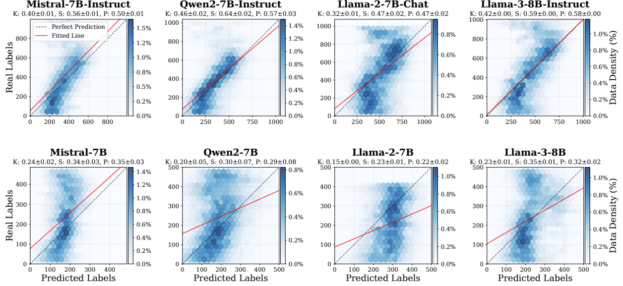
(a) UltraChat to AlpacaEval generalization for response length prediction.
