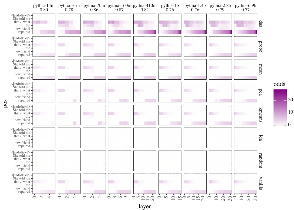
Figure 11: filler_gap_obj
