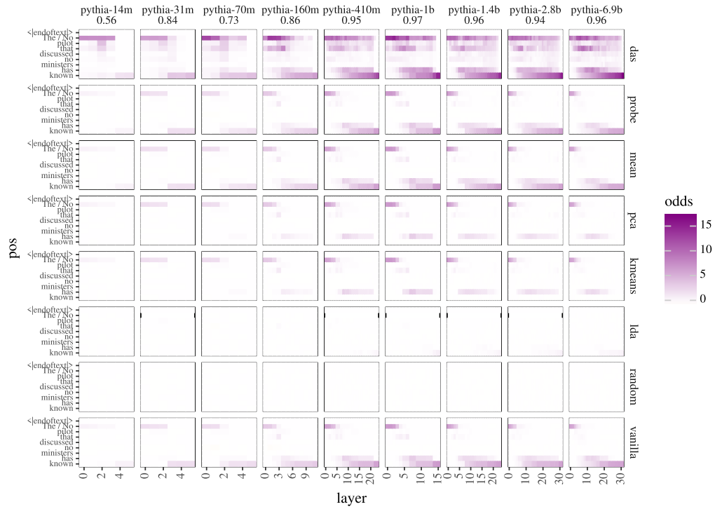
Figure 9: npi_any_subj-relc
