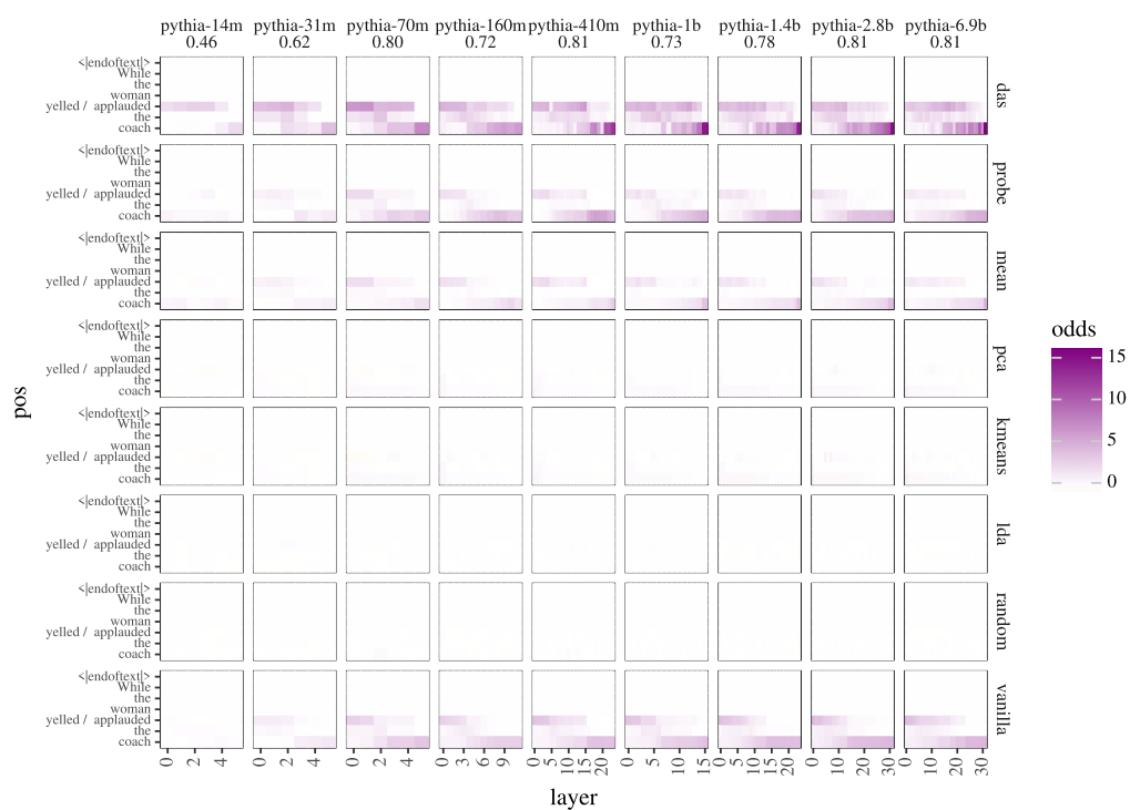
Figure 10: garden_npz_v-trans
