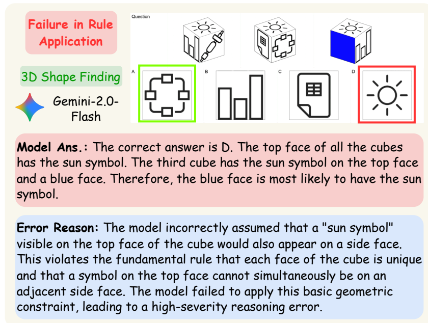
Figure 12: Error example of Failure in Rule Application
