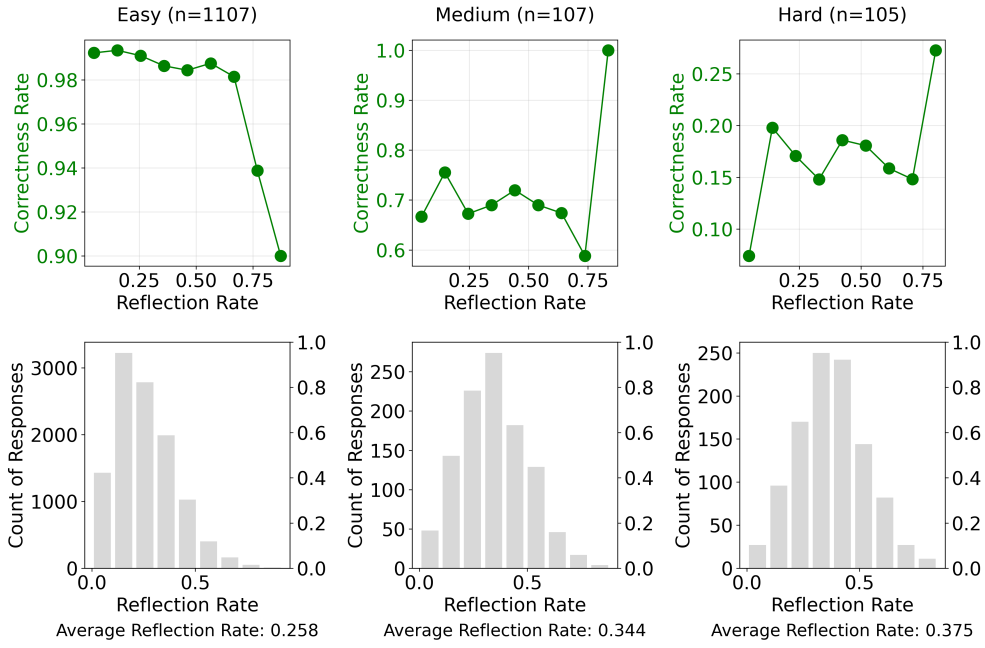
(a) Base model. Top: Correctness rate vs. reflection rate. Bottom: Reflection rate distribution.
