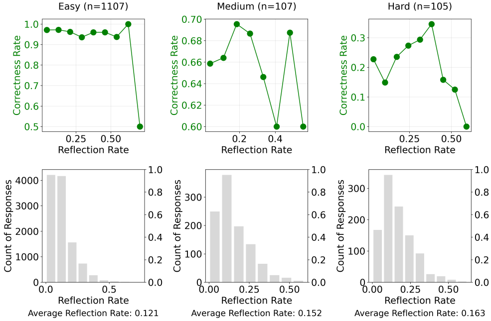
(b) Intervention. Top: Correctness rate vs. reflection rate. Bottom: Reflection rate distribution.
