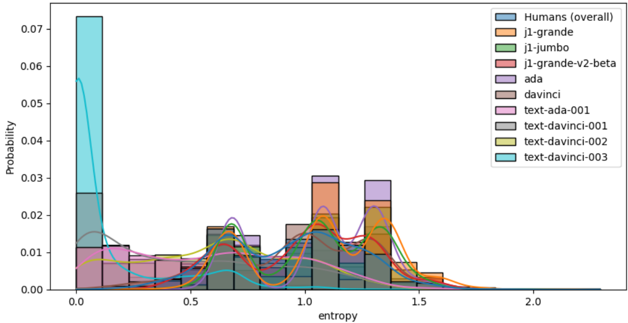
Figure 9: A comparison of the entropy of LM response distributions: text-davinci-003 tends to assign most of it's probability mass to a single option. This is in contrast to human opinions which tend to have a fair amount of variability.
