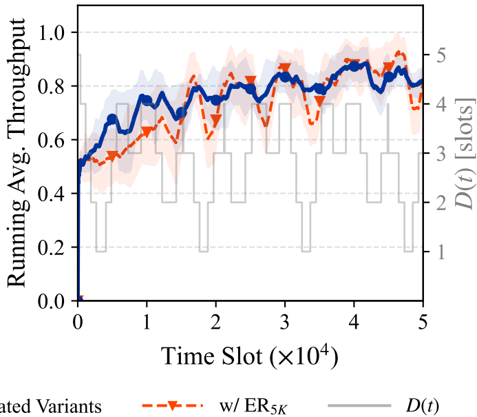
(b) Mobility adaptation: STER vs. ER
