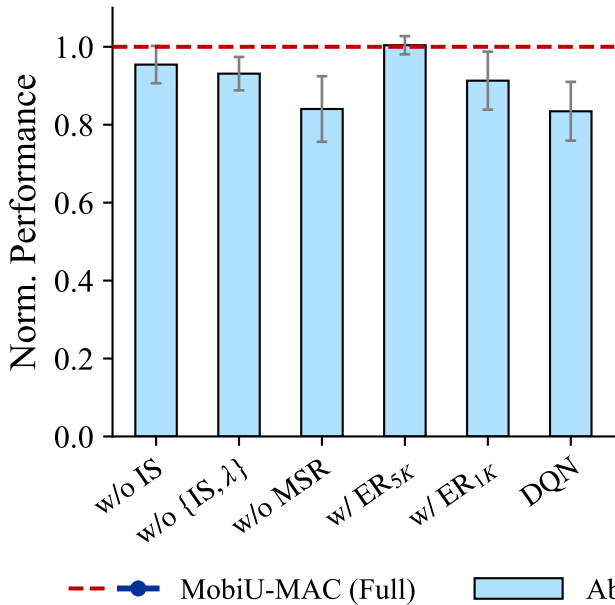
(a) Component ablation analysis
