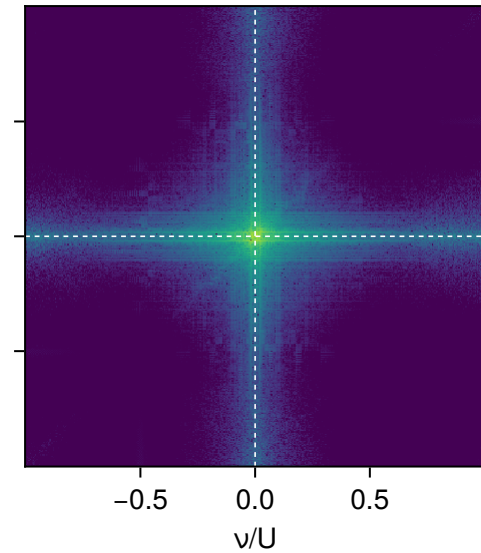
\eta = 2: \log_{10}(|F_{\text{code}} - F_{(3)}| / \max|F_{(3)}|)
