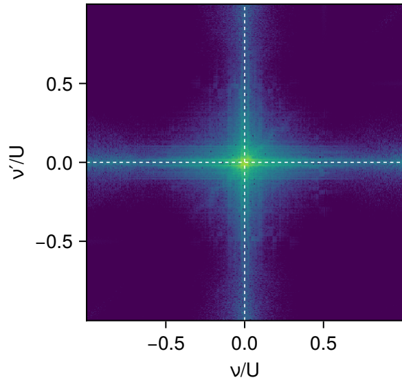
\eta = 1: \log_{10}(|F_{\text{code}} - F_{(3)}| / \max|F_{(3)}|)
