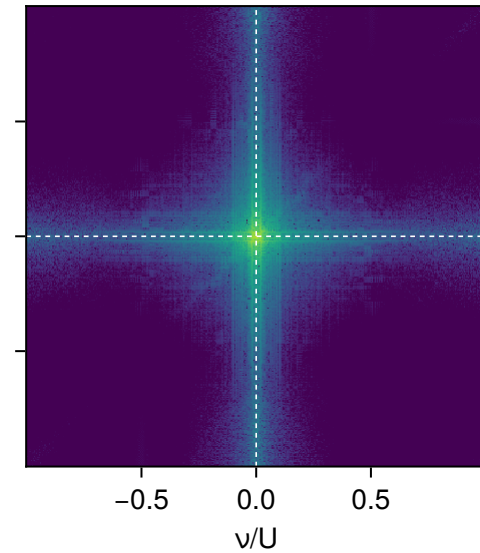
\eta = 3: \log_{10}(|F_{\text{code}} - F_{(3)}| / \max|F_{(3)}|)
