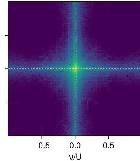
\eta = 4: \log_{10}(|F_{\text{code}} - F_{(3)}| / \max|F_{(3)}|)
