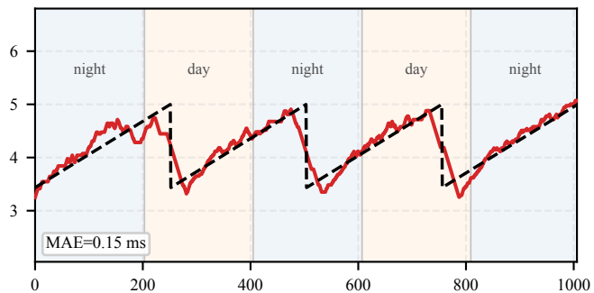
Sawtooth budget
