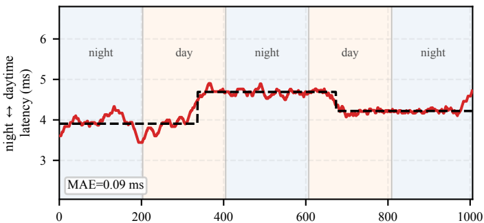
Step budget
