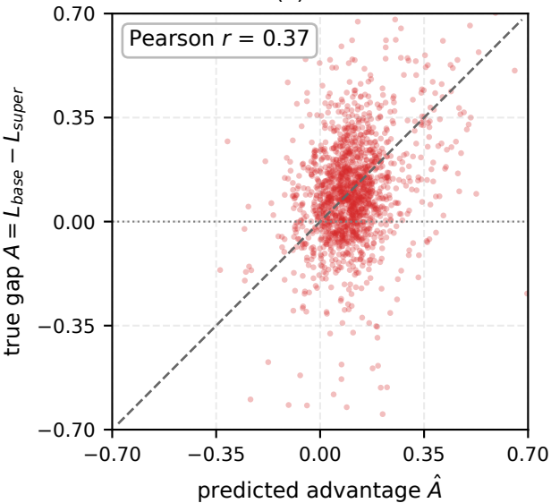
(a) KITTI
