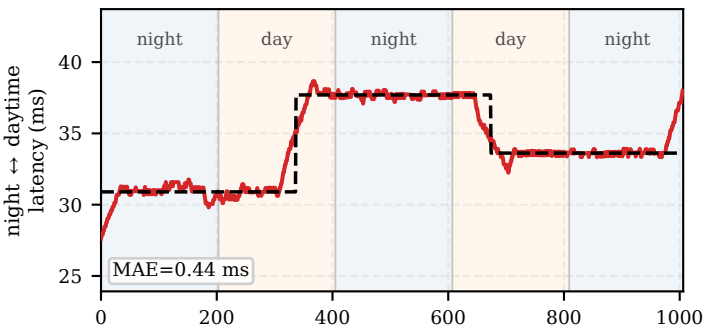
Step budget
