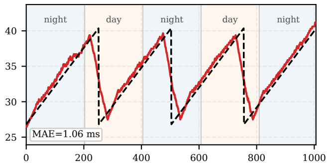
Sawtooth budget
