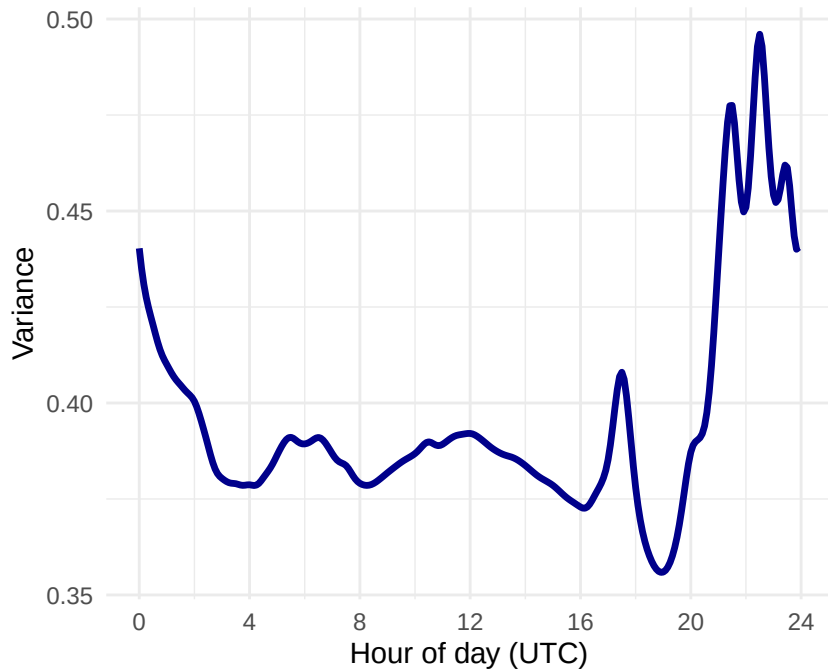
Variance function
