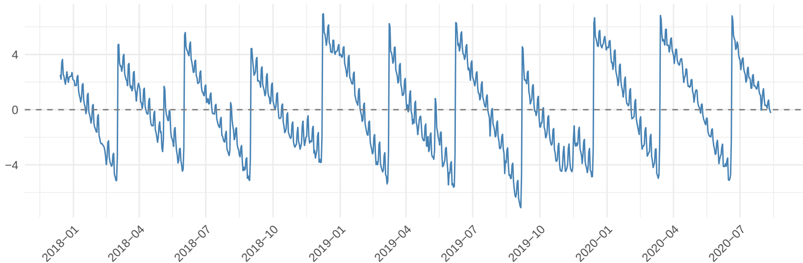
FPC1 score
