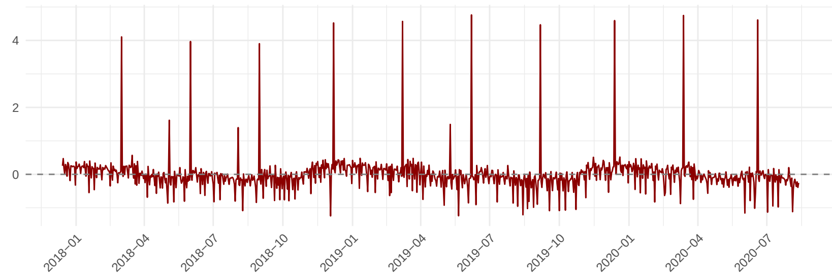
FPC2 score
