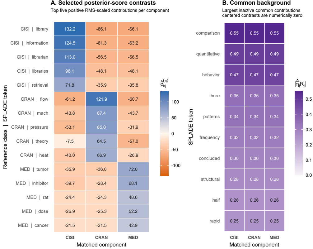
Figure 4: E-CGL coordinate interpretation in Classic3. E-CGL selected 1,421 of 2,000 coordinates. Panel A shows signed centered natural-parameter coefficients for coordinates selected by their positive root-mean-square-scaled contribution to each matched component (blue positive, orange negative). Panel B shows the ten inactive coordinates with the largest absolute common root-mean-square-scaled contribution; their near-identical component values illustrate a retained common background rather than posterior-score heterogeneity. Supplied labels were used only after fitting to align and name components.
