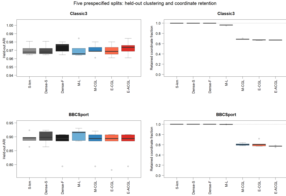
Figure S3: Five prespecified splits: held-out ARI and coordinate-retention distributions. Coordinate retention is interpreted relative to each method-specific support target. The Classic3 E-CGL values coincide under its primary standard path and the augmented audit, whereas E-ACGL uses the final augmented candidate rule. BBCSport retains the common standard E-series path.
