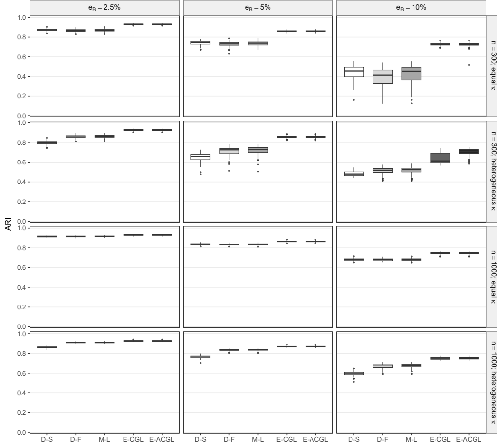
Figure S1: Adaptive sensitivity display for the primary simulation grid: repetition-level ARI distributions including E-ACGL. D-S and D-F denote dense shared- and free-concentration vMF mixtures. The E-ACGL values correspond to the final augmented rerun; they are retained here rather than in the main article because E-ACGL is a supplementary extension.
