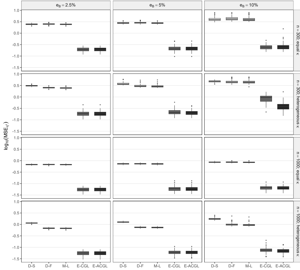
Figure S2: Adaptive sensitivity display for the primary simulation grid: repetition-level \log_{10}(\text{MSE}_{\eta^c}) distributions including E-ACGL. The archived standard path and final augmented path selected the same support in all 1,200 primary E-ACGL repetitions.
