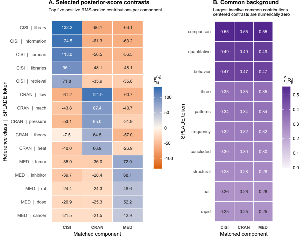
Figure 4: Selected posterior-score contrasts and retained common effects in Classic3. E-CGL selected 1,421 of 2,000 coordinates. Panel A shows signed centered natural-parameter coefficients for coordinates ranked by I_{kj}^{(\eta)} = \hat{c}_{kj}R_j (blue, positive; orange, negative). Panel B shows the ten inactive coordinates having the largest I_j^{(\text{com})} = |\hat{\eta}_jR_j| . Their equal component values represent retained common effects rather than posterior-score heterogeneity. Supplied labels were used only after fitting to align and name the components.
