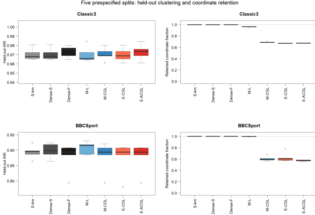
Figure S1: Clustering accuracy and coordinate retention across the five prespecified real-data splits. Coordinate retention is defined relative to each method-specific support target. E-CGL and E-ACGL use the final single 240-point KKT-motivated path in both datasets; M-CGL uses its 240-point dense-score-proxy path, and M-L retains its event-driven path.
