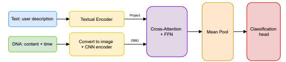
Fig. 1: Text-DNA Cross-Attention bot detection framework.
