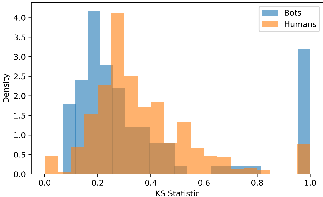
KS Test: Gamma
