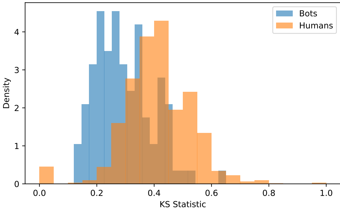
KS Test: Normal
