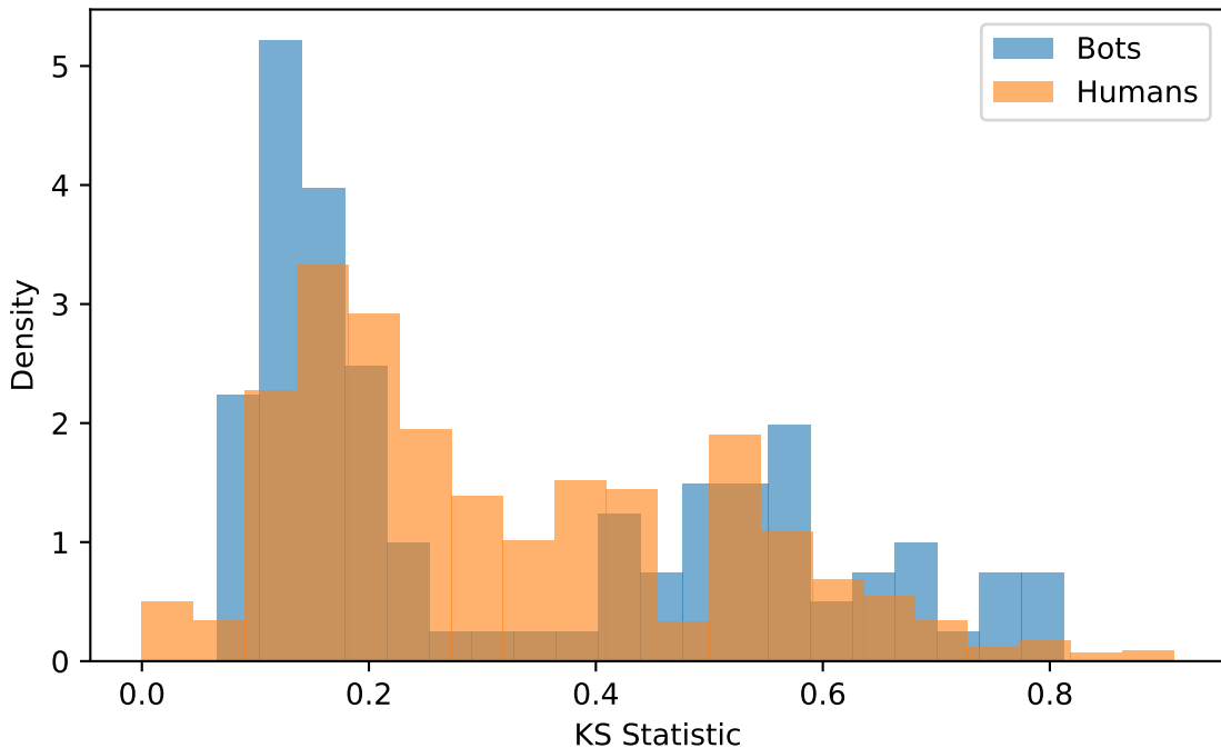
KS Test: Pareto
