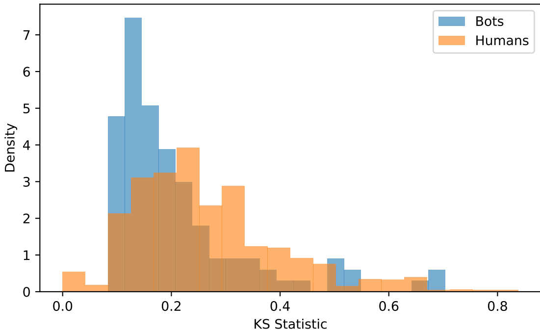
KS Test: Loglogistic
