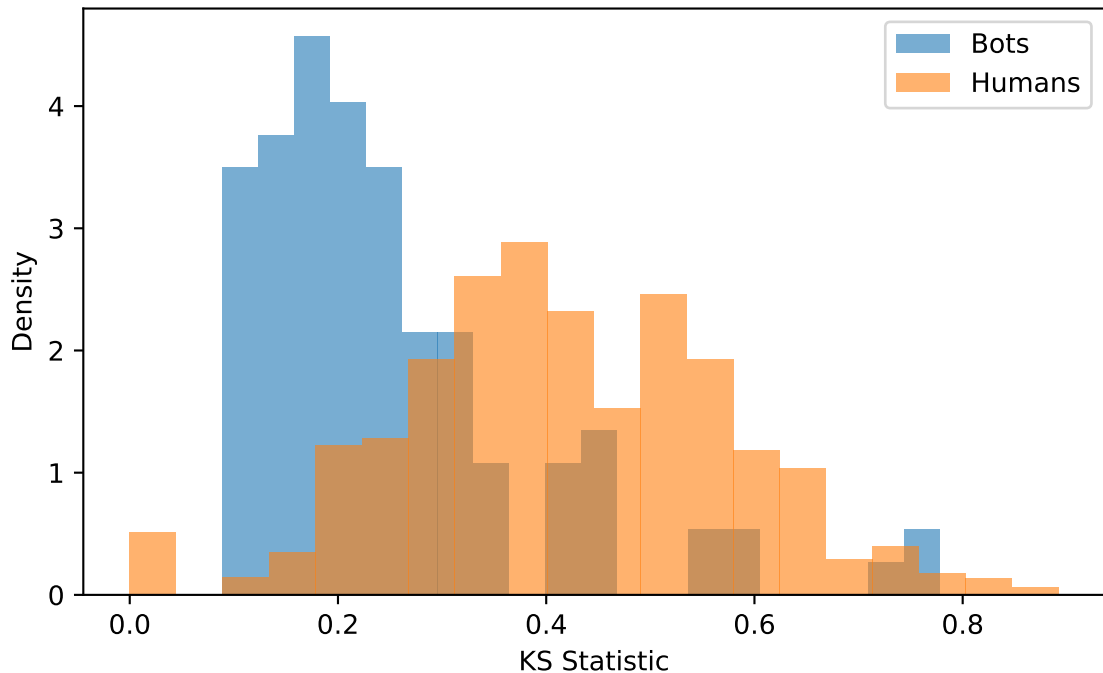
KS Test: Ks Exponential
